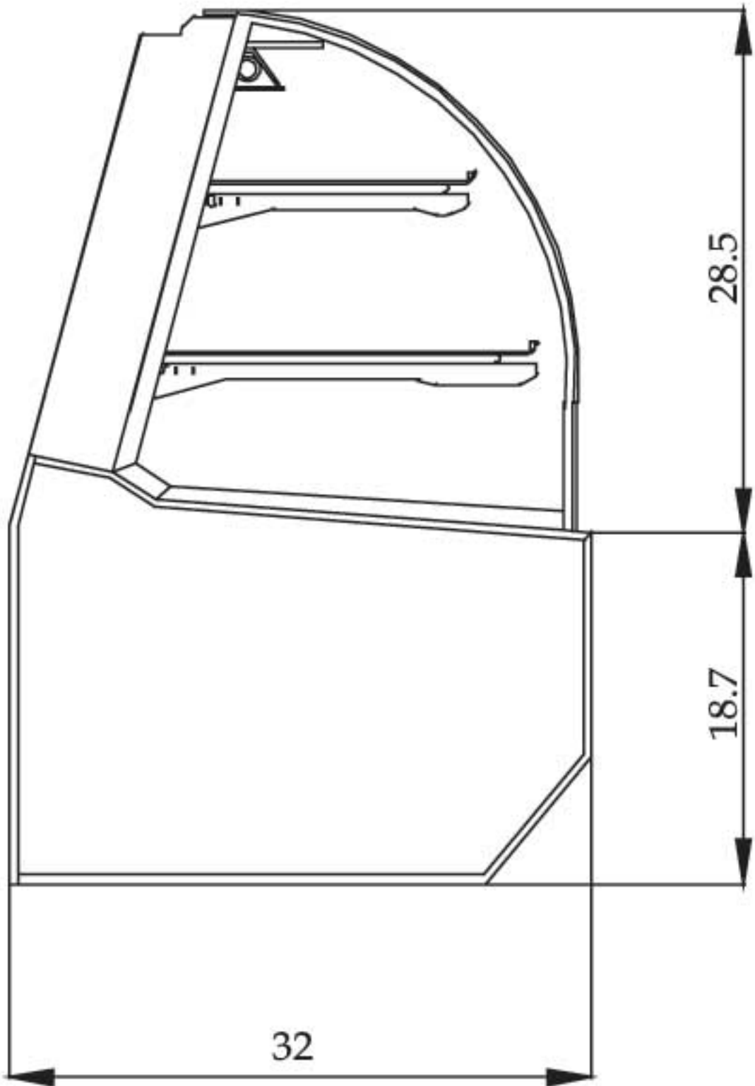
SIDE VIEW
