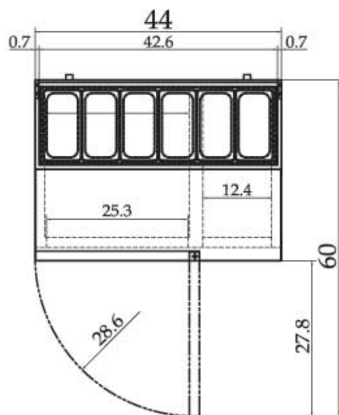
TPR-44SD PLAN VIEW
