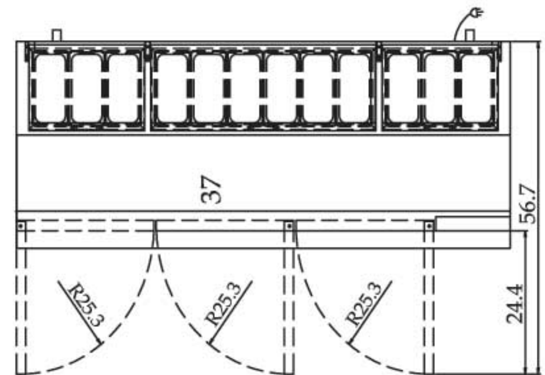
TPR-93SD PLAN VIEW
