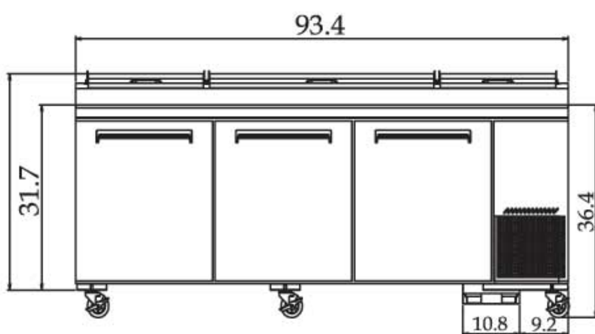
TPR-93SD FRONT VIEW
