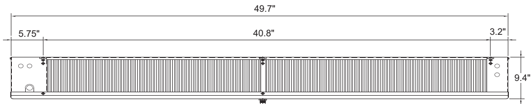
FRONT VIEW
