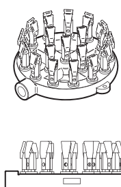
BURNER DUCK ASSY
