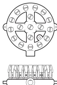
BURNER DUCK ASSY
