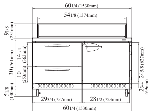
PST-60-24-D2R-FB-N FRONT VIEW
