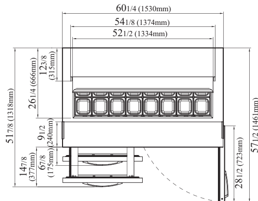
PST-60-24-D2R-FB-N TOP VIEW
