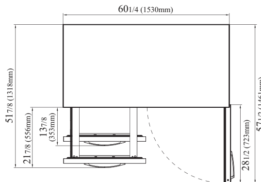
PUR-60-D2R-FB-N TOP VIEW
