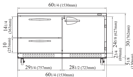
PUR-60-D2R-FB-N FRONT VIEW
