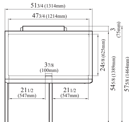
M3F47-2-N-AL TOP VIEW
