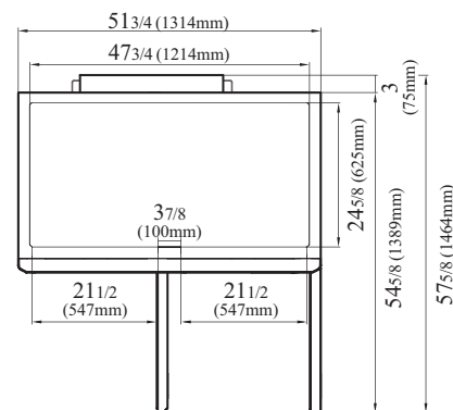
M3F47-2-N-AR TOP VIEW
