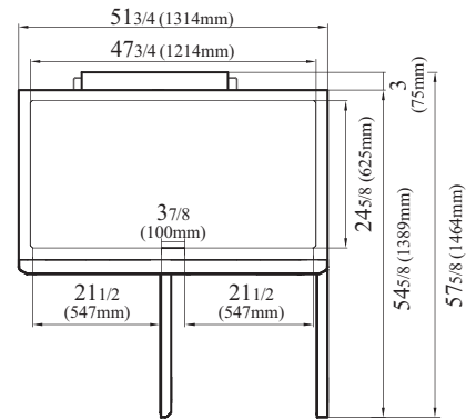
M3F47-2-N-AR TOP VIEW
