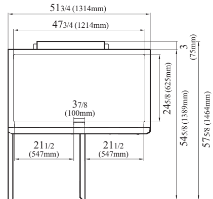
M3F47-2-N-AL TOP VIEW
