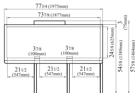
M3F72-3-N-AR TOP VIEW
