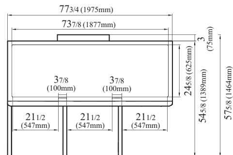
M3F72-3-N-AL TOP VIEW
