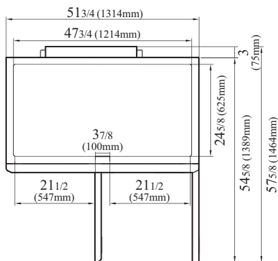
M3R47-2-N-AR TOP VIEW
