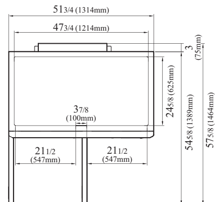
M3R47-2-N-AL TOP VIEW
