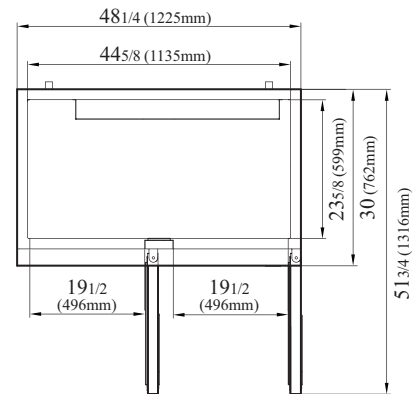
TUR-48SD-N-AR TOP VIEW
