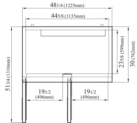
TUR-48SD-N-AL TOP VIEW
